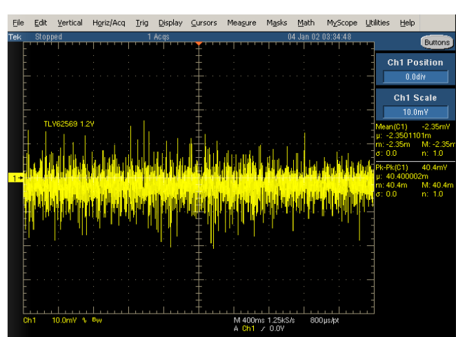
Fig6: TLV62569DRLR_P1V2_ripple
