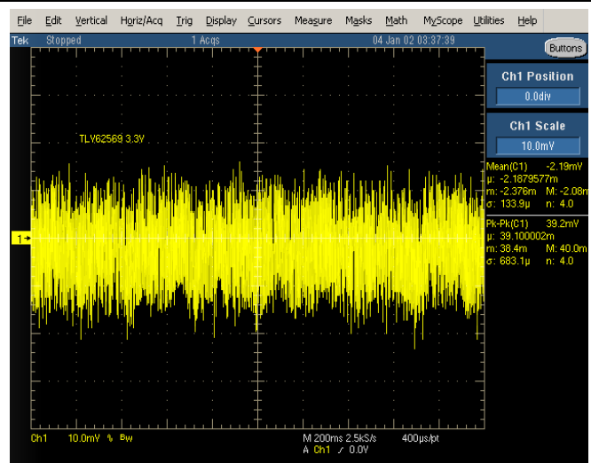
Fig8: TLV62569DRLR _P3V3_ripple
